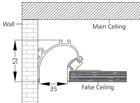
Cove Asymmetric M #2073
