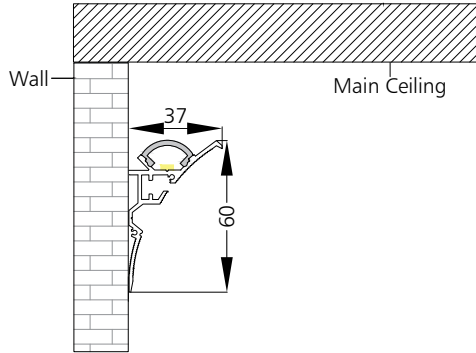
Cove Uplight M #2075
