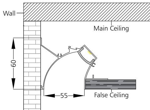
Cove Asymmetric L #2071
