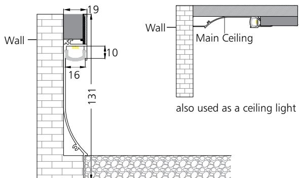
Floor Curve M #2079
