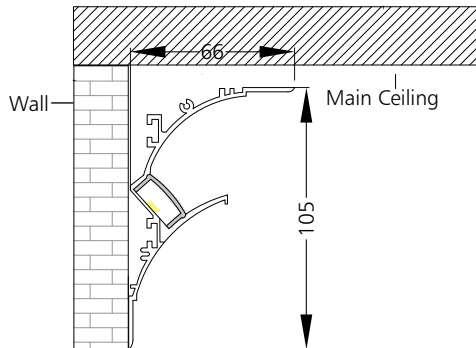
Cove Uplight L #2076
